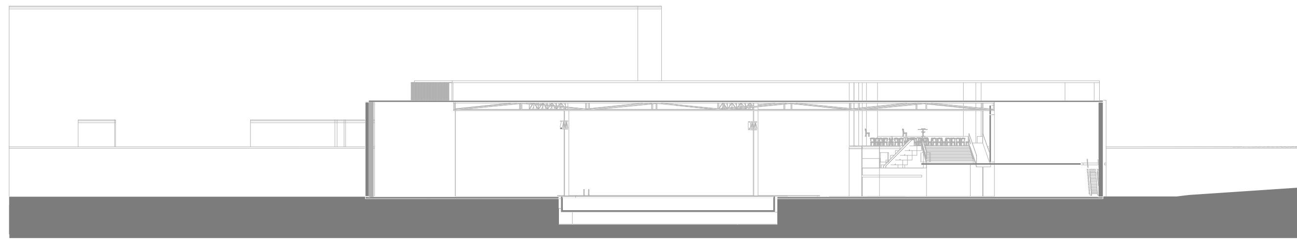
SECTION D-D'
